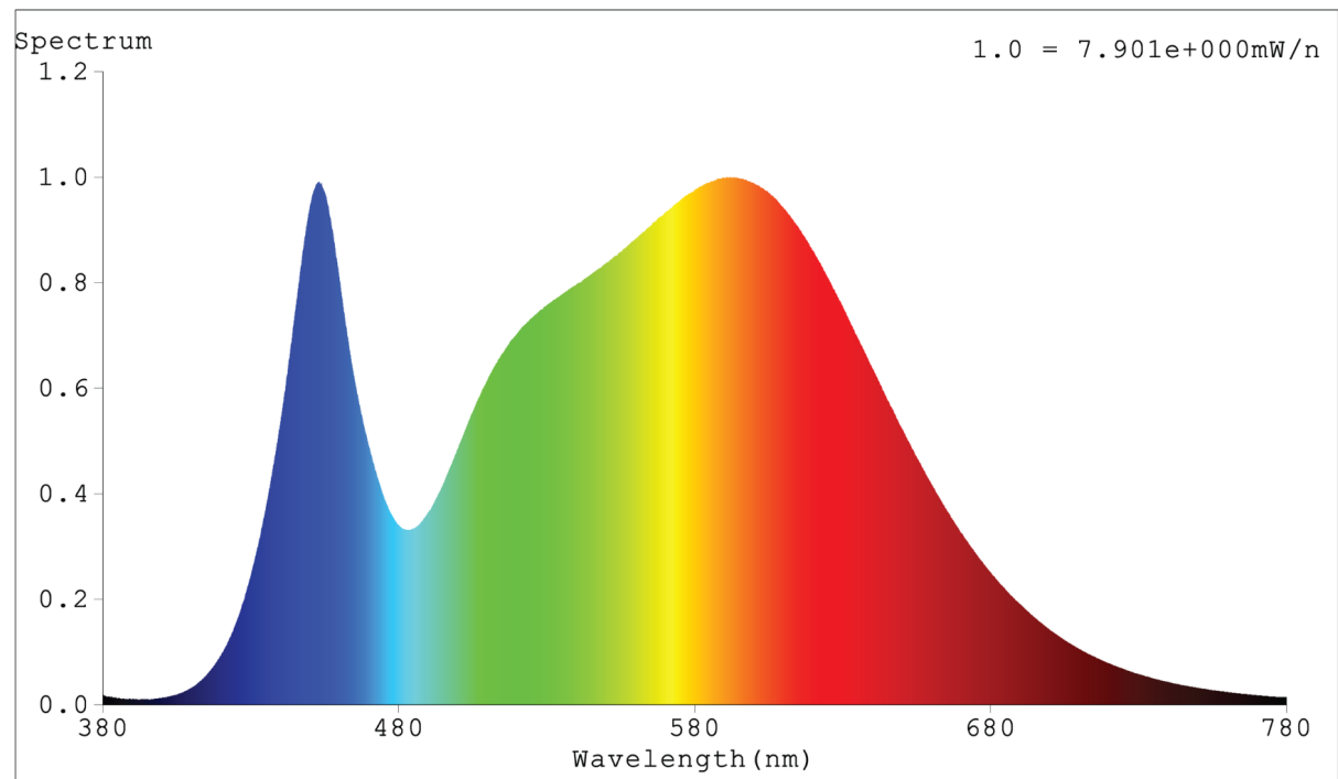
Spectral Distribution
